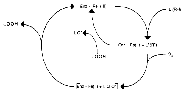
Scheme I: Catalytic Cycle of the Dioxygenation of Linoleic Acid (LH) by Soybean Lipoxygenase [Enz-Fe(III) or Enz-Fe(II)] and Catalytic Cycle of the Oxidation of Lipoxygenase Inhibitors (RH) by Soybean Lipoxygenase and 13-HPOD (LOOH)
