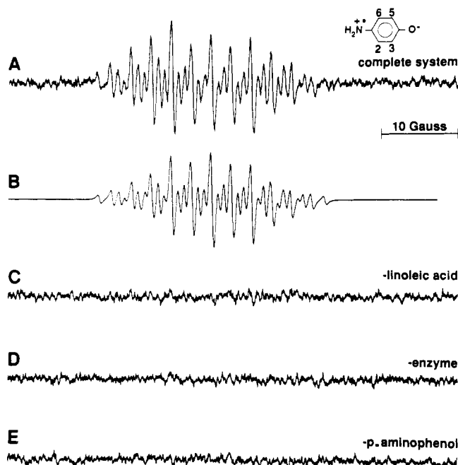
FIGURE 4: Oxidation of p -aminophenol. (A) The reaction mixture contained p -aminophenol (2 mM), lipoxigenase (55 \mu\text{g/mL} ), and linoleic acid (0.83 mM) in 0.1 M sodium phosphate buffer, pH 6.5, containing 1 mM DETAPAC. Instrumental conditions were as follows: microwave power, 20.9 mW; modulation amplitude, 0.5 G; time constant, 0.66 s; scan range, 60 G; scan time, 5 min. (B) Simulation of spectrum in (A). Hyperfine splitting constants were a^{\text{H}}_{\text{N}} = 5.4 G, a^{\text{H}}_{\text{NH}_2} = 5.25 G (2 H), a^{\text{H}}_{\text{ortho}} = 2.77 G (2 H), and a^{\text{H}}_{\text{meta}} = 1.74 G (2 H). Line width = 0.4 G. (C) As (A), but no linoleic acid. (D) As (A), but no lipoxigenase. (E) As (A), but no p -aminophenol.
