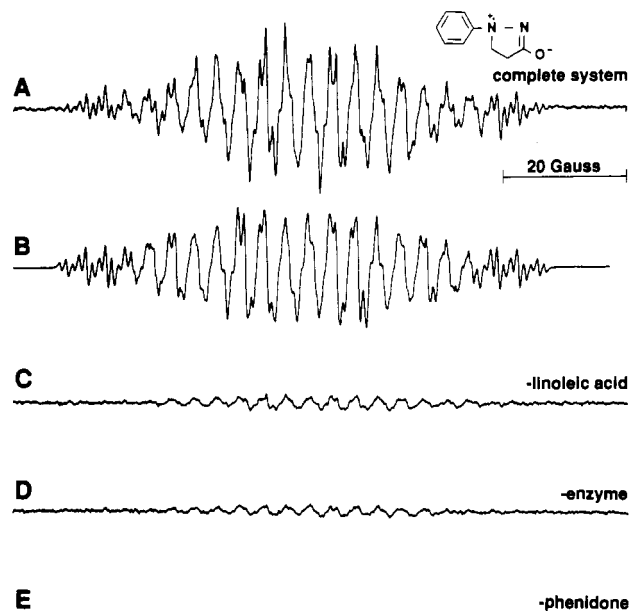
FIGURE 1: Oxidation of phenidone. (A) The incubation mixture contained phenidone (0.52 mM), lipoxygenase (57 \mu\text{g}/\text{mL} ), and linoleic acid (0.86 mM) in 0.1 M sodium phosphate buffer, pH 6.5, containing 1 mM DETAPAC. Instrumental conditions were as follows: microwave power, 20.9 mW; modulation amplitude, 0.5 G; time constant, 0.66 s; scan width, 100 G; scan time, 5 min. (B) Simulation of spectrum in (A). Hyperfine splitting constants were a_1^N = 14.9 G, a_2^N = 7.42 G, a_{\text{CH}_2}^H = 11.5 G (2 H), a_{\text{ortho}}^H = 3.17 G (2 H), a_{\text{meta}}^H = 1.05 G (2 H), and a_{\text{para}}^H = 3.47 G. Line width = 0.4 G. (C) As (A), but no linoleic acid. (D) As (A), but no lipoxygenase. (E) As (A), but no phenidone.
