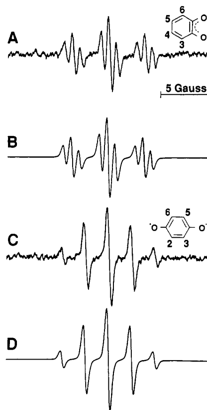
FIGURE 5: Oxidation of catechol and hydroquinone. (A) The reaction mixture contained catechol (2 mM), lipoxigenase (57 \mu\text{g/mL} ), and linoleic acid (0.83 mM) in 0.1 M sodium phosphate buffer, pH 6.5, containing 1 mM DETAPAC. Instrumental conditions were as follows: microwave power, 20.9 mW; modulation amplitude, 0.5 G; time constant, 0.66 s; scan range, 40 G; scan time, 5 min. (B) Simulation of spectrum in (A). Hyperfine splitting constants were a^{\text{H}}_{4,5} = 3.68 G (2 H) and a^{\text{H}}_{3,6} = 0.77 G (2 H). Line width = 0.3 G. (C) As (A), but with hydroquinone (2 mM). (D) Simulation of spectrum in (C). Hyperfine splitting constant was a^{\text{H}}_{2,3,5,6} = 2.36 G (4 H). Line width = 0.3 G.
